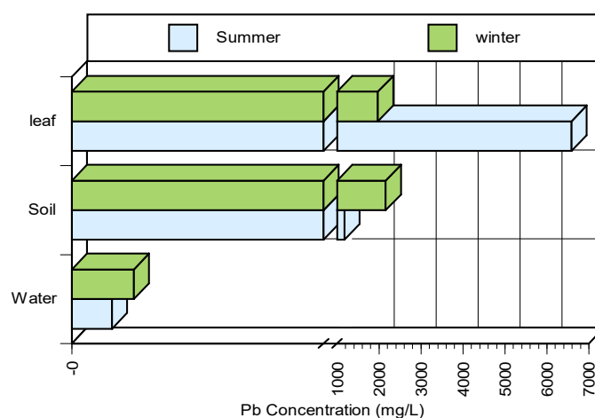
Figure 3: Lead (Pb) concentration at different environmental compartments of the study area.
