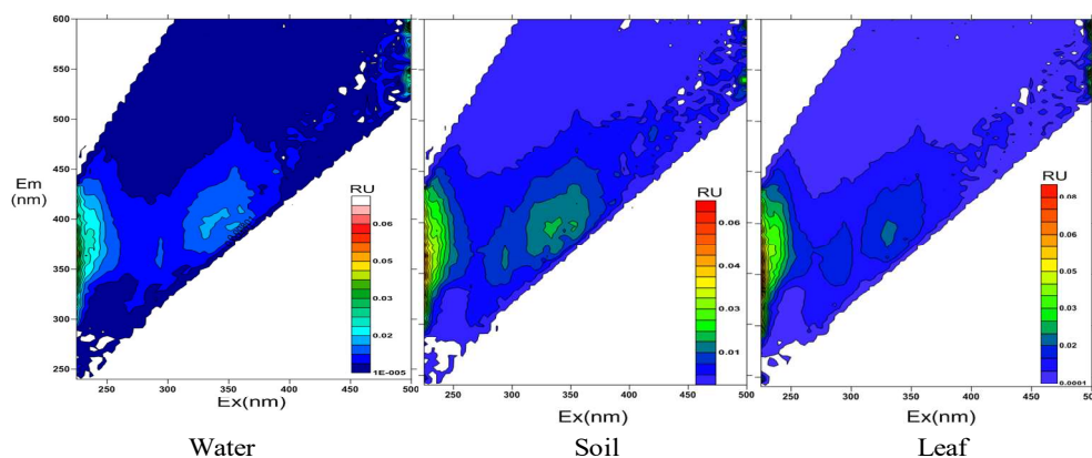
Figure 2: EEM plots of surface water, soil and blackish materials of plant leaf samples.
