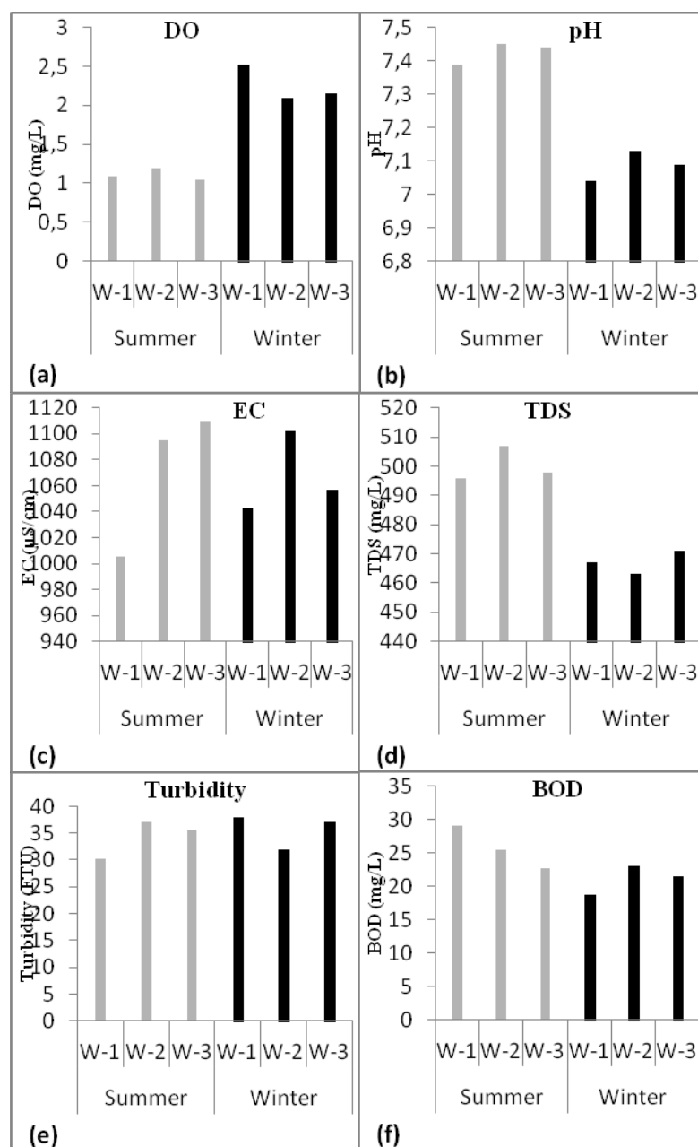
Fig 1: Physicochemical parameters of water samples of the study area.
